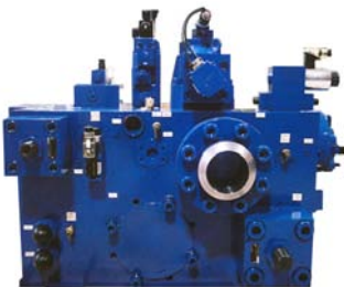
3000 ton press main manifold utilizing Parker Valves
