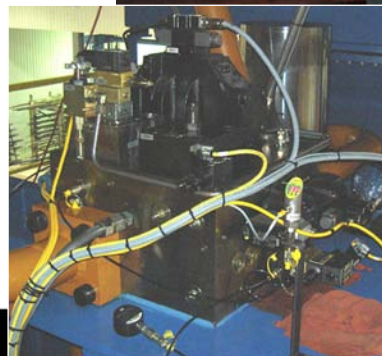
3000 ton press main manifold utilizing Parker Valves
